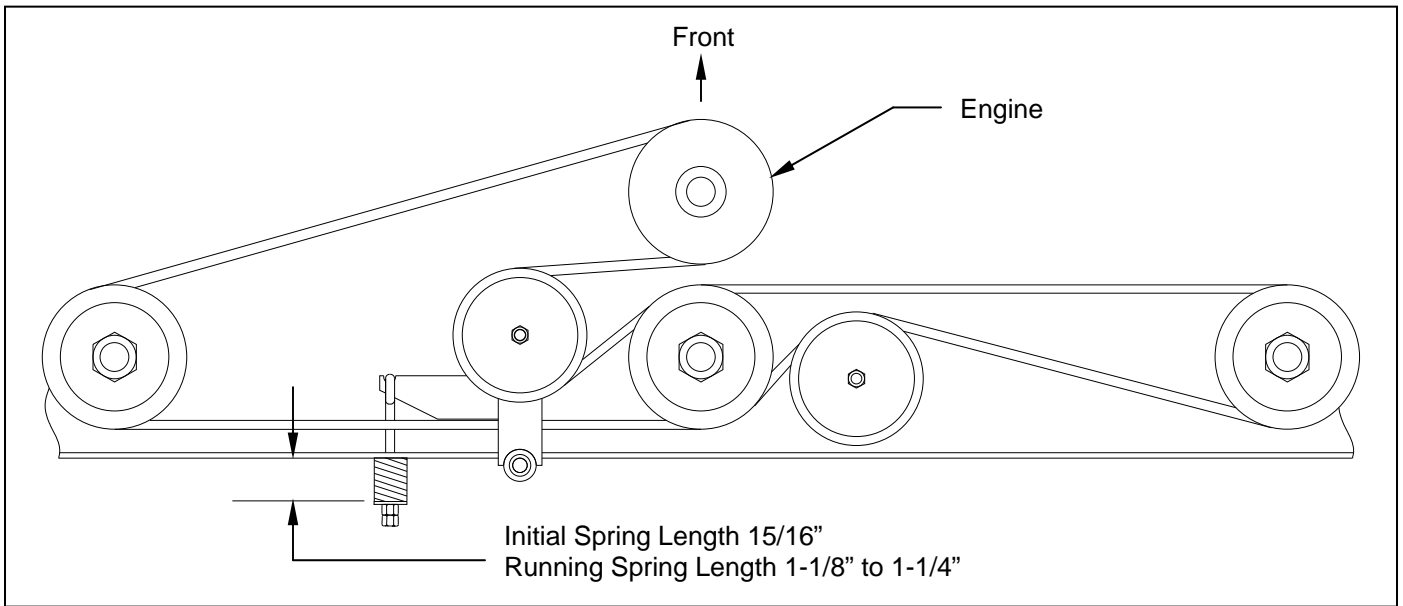
Figure 9: Belt Pattern and Spring Adjustment (Model C60V)
